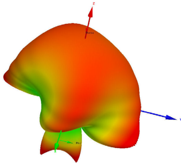
Fig 17 – Axial Ratio in 3D
