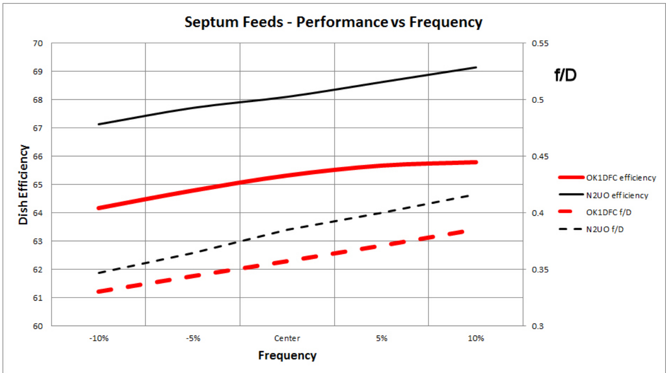
Figure 8 - Septum Feed antenna performance vs frequency
