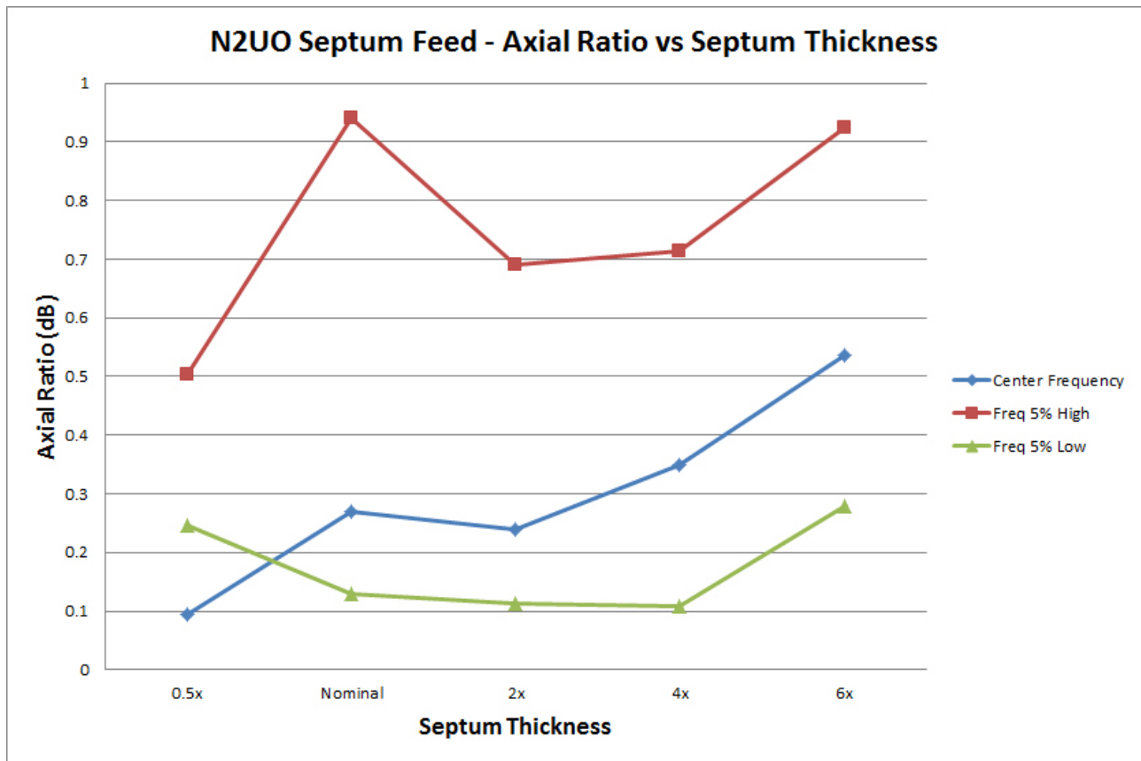
Figure 6 – N2UO Septum Feed Sensitivity to septum thickness
