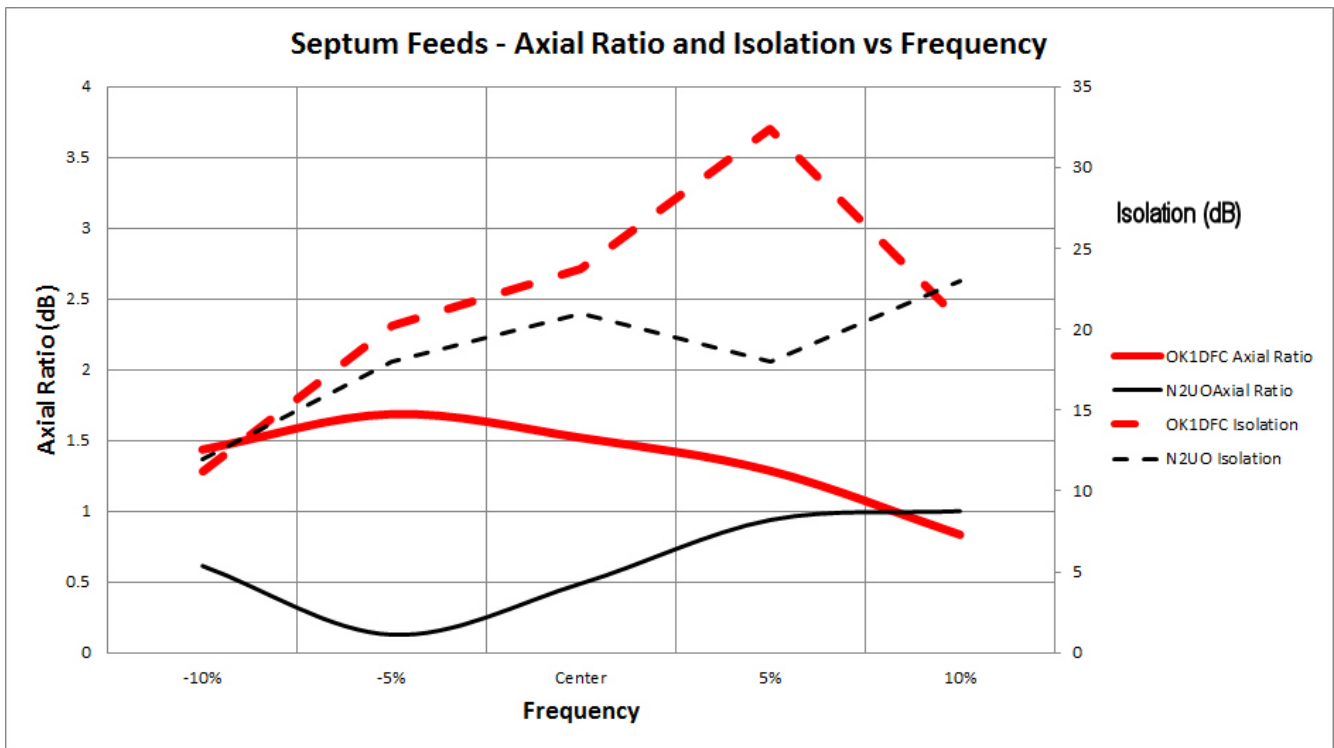
Figure 7 – Axial Ratio and Isolation over frequency range
